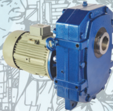
Parallel Helical Geared Motor
